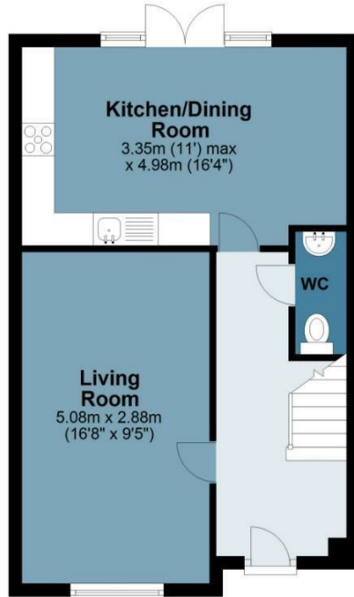
Ground Floor Approx. 39.2 sq. metres (422.1 sq. feet)
